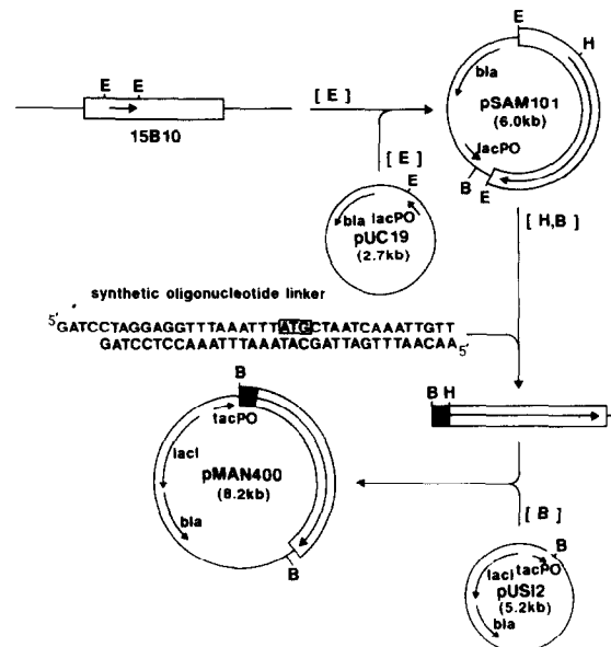
Fig.1. Construction of pMAN400 carrying the highly-expressible secA gene. The open box denotes chromosomal DNA. The arrow in the open box shows the coding region and the direction of transcription of the secA gene. The closed box denotes the synthetic oligonucleotide linker. The initiation codon ATG of the secA gene is boxed. The restriction endonucleases used are shown in parentheses with the following abbreviations: E, EcoRI ; H, HpaI ; B, BamHI . Cleavage sites are also shown.
